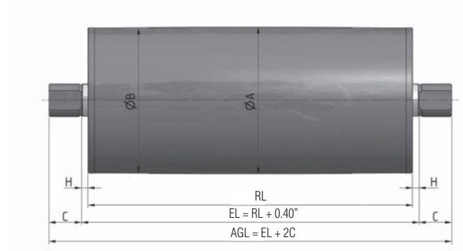
Idler Pulley.
