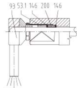
Electromagnetic brake
