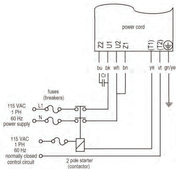
Low Voltage - Counterclockwise Rotation
