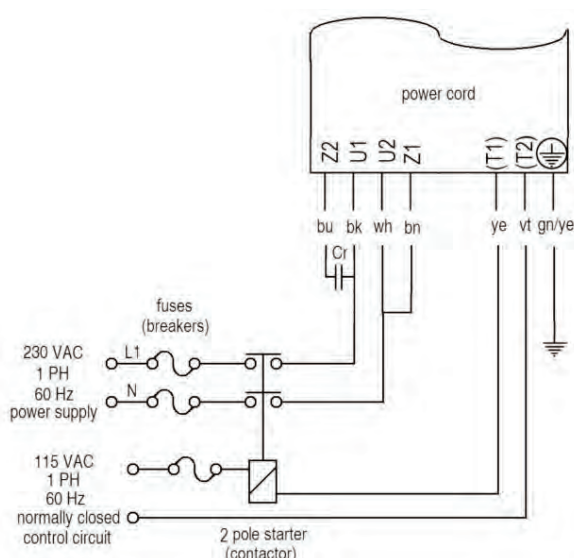
High Voltage - Counterclockwise Rotation
