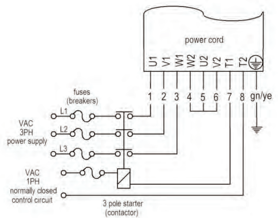
High Voltage
