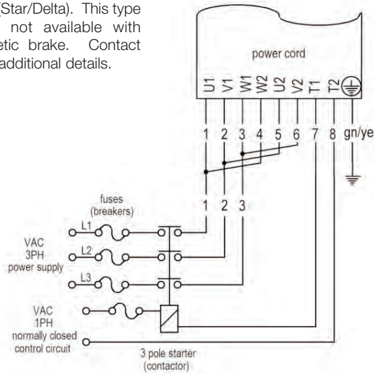
Low Voltage
