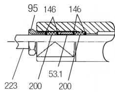
Electromagnetic Brake Option
