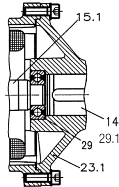
Mechanical Backstop Option
