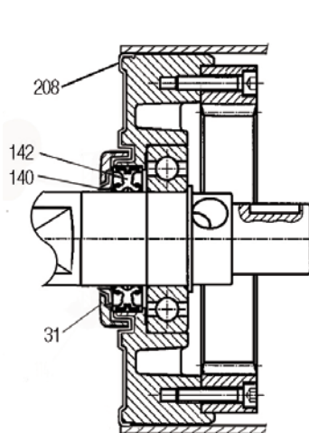
Stainless steel end housing
